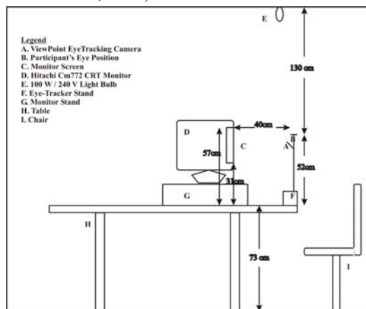
Figure 1: The layout of the experimental room.
